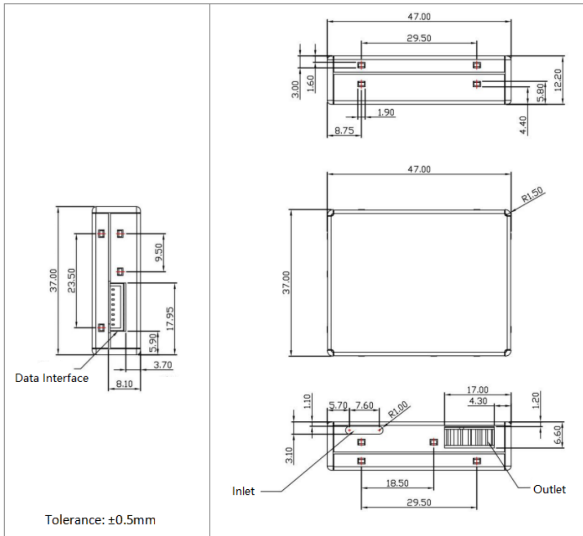
Fig4. Sizes
